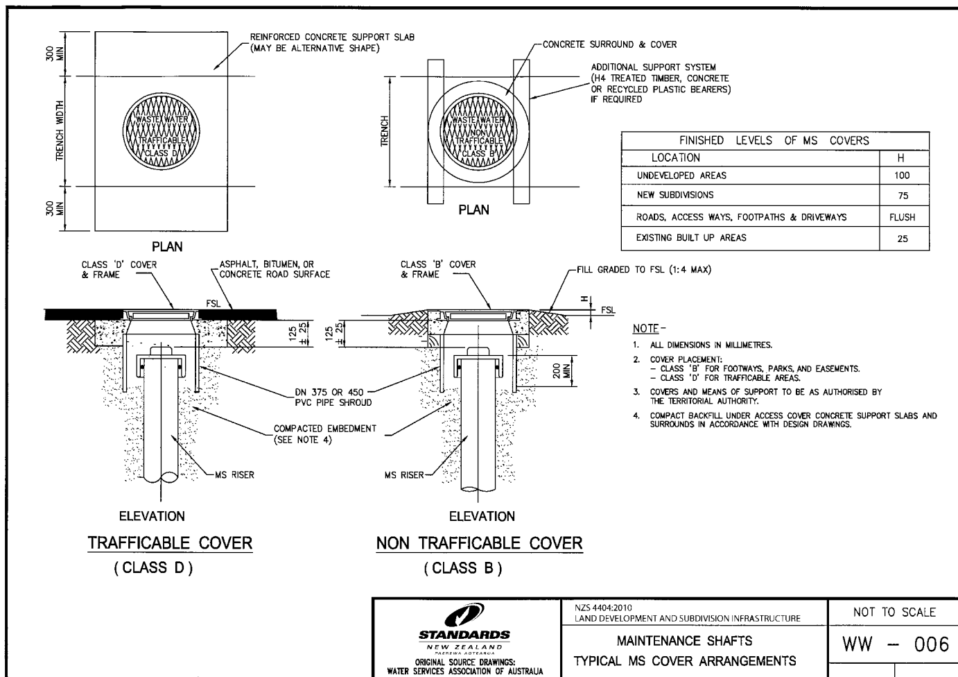
WW - 006 Maintenance shafts - Typical MS cover arrangements
