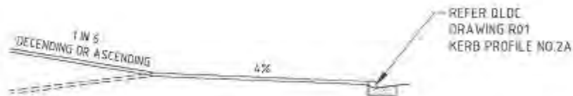
SECTION X-X
