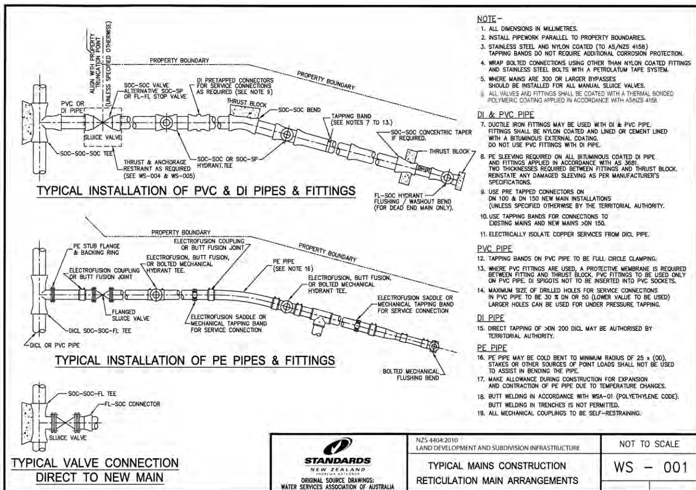
WS - 001 Typical mains construction - Reticulation main arrangements
