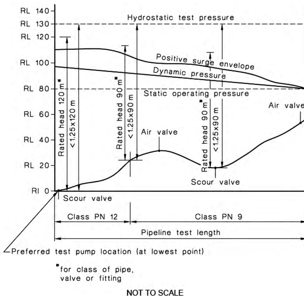
Figure C1 – Typical pressure pipeline under field hydrostatic test
