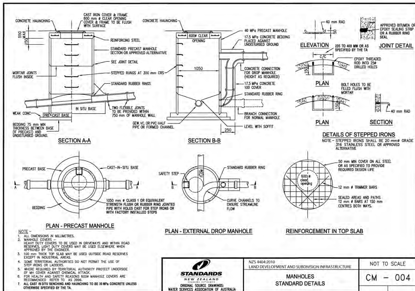
CM - 004 Manhole - Standard details
