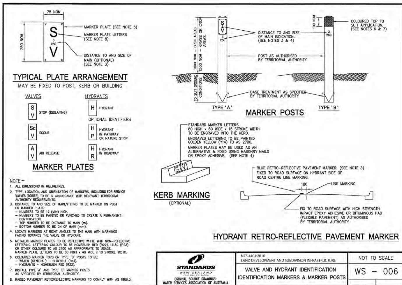
WS – 006 Valve and hydrant identification – Identification markers and marker posts
