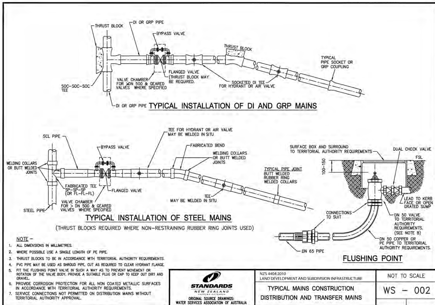
WS - 002 Typical mains construction - Distribution and transfer mains
