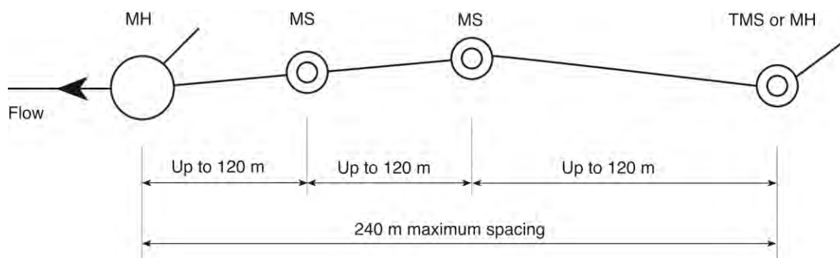
Figure 5.1 – Multiple MSs between MH and ‘last’ MH/TMS
