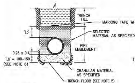
TYPE 1 SUPPORT
