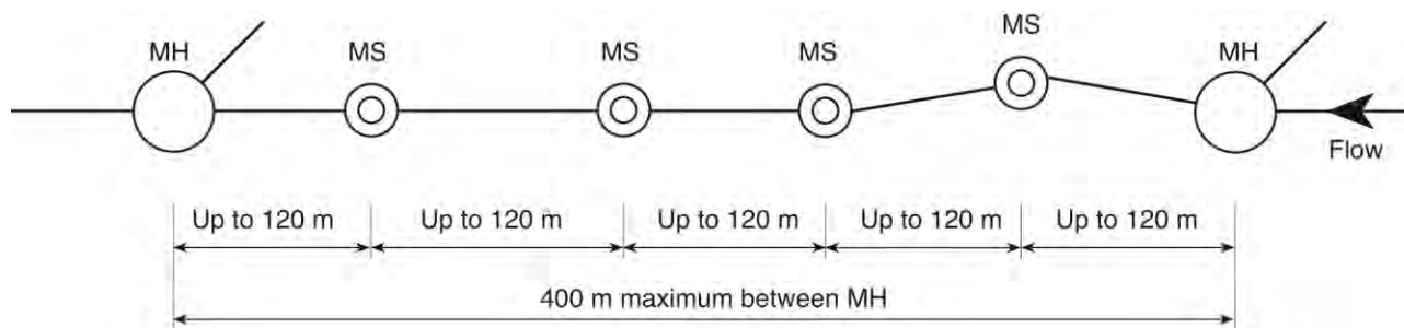
Figure 5.2 – Multiple MSs between consecutive MHs
