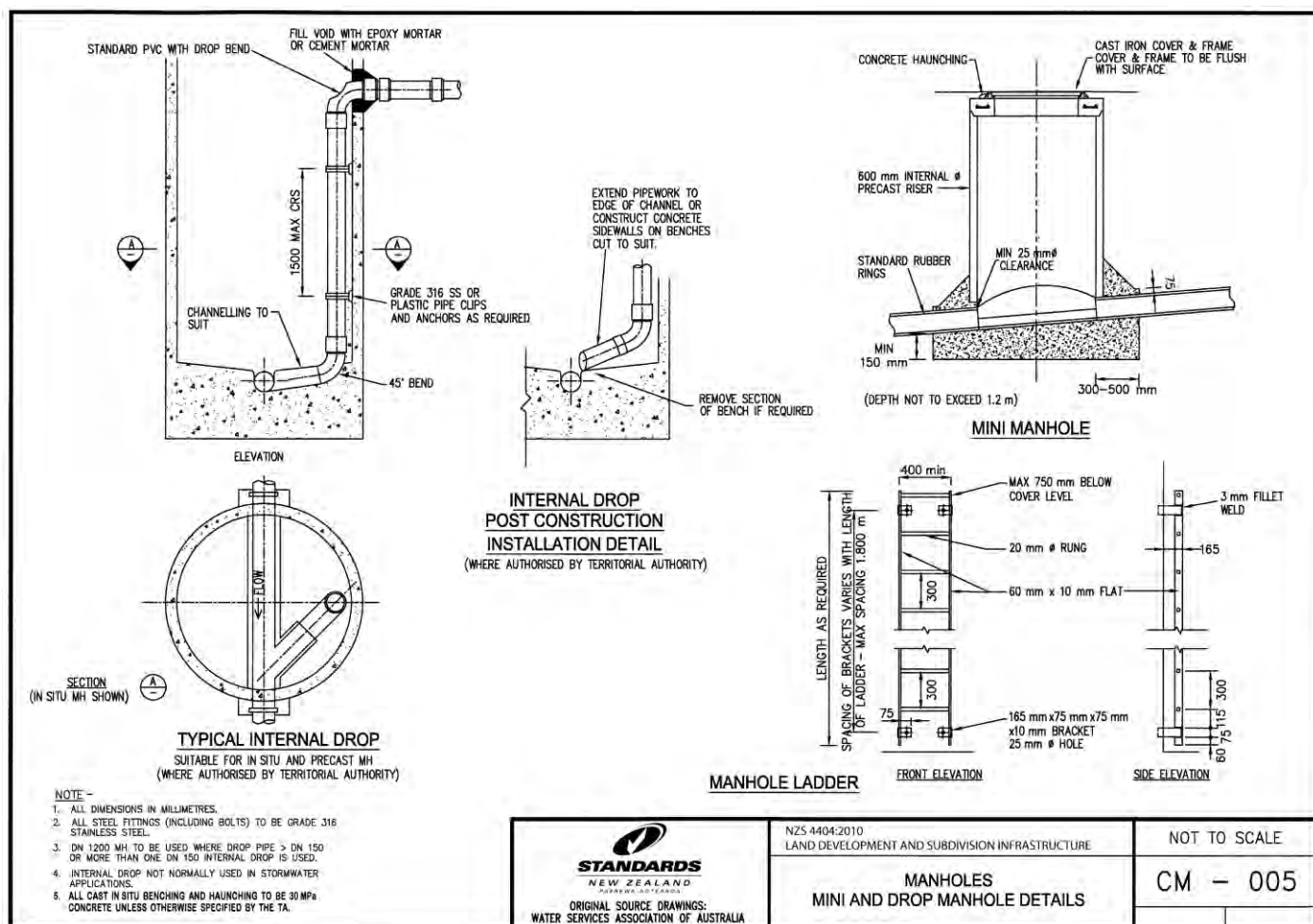
CM – 005 Manholes – Mini and drop manhole details
