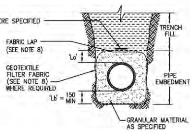
TYPE 4 SUPPORT
