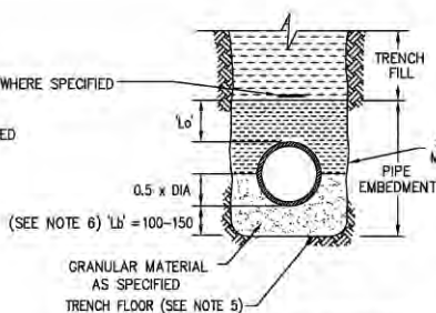
TYPE 2 SUPPORT
