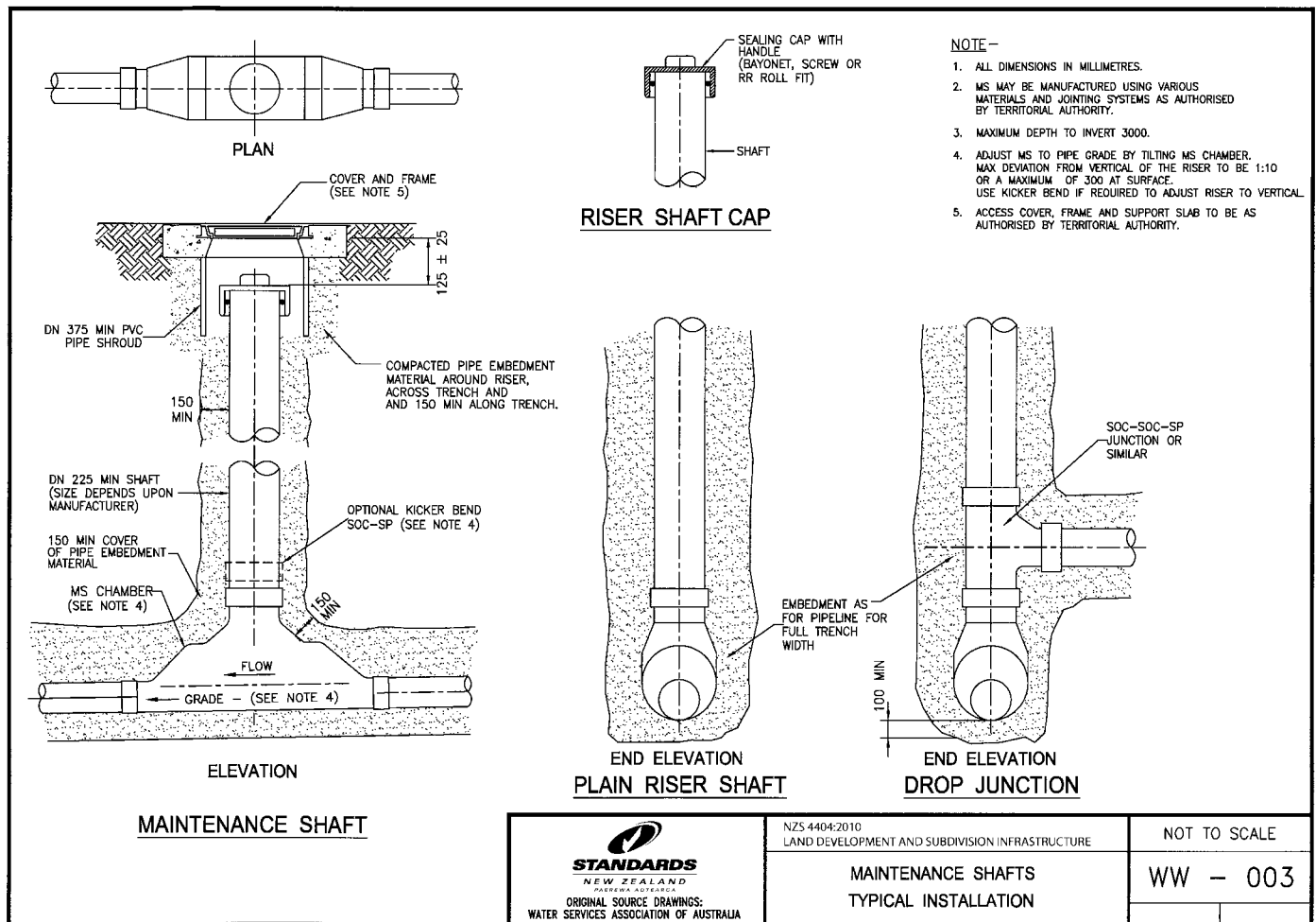
WW - 003 Maintenance shafts - Typical installation
