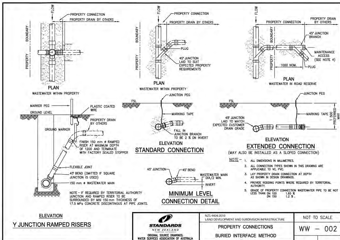
WW – 002 Property connections – Buried interface method
