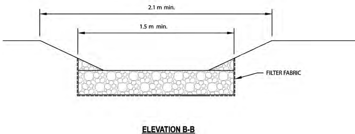
Figure 3.6(C) – Typical check dam detail
