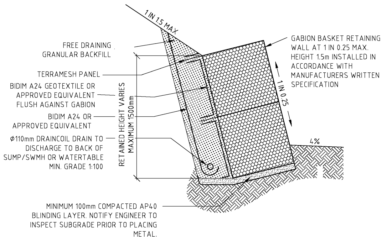
Drawing B5-30: Low Retaining Wall: Gabion
