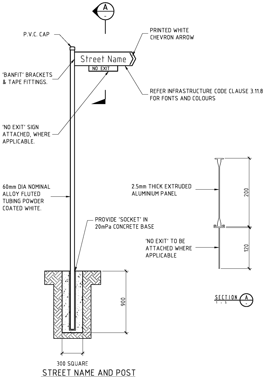
Drawing B6-3: Street Sign: Pole Mounted
