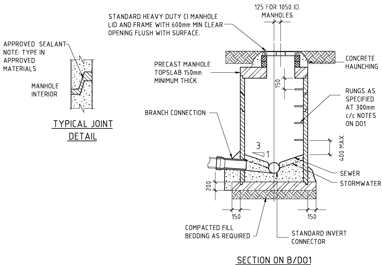
Drawing B1-6 Manhole Details B
