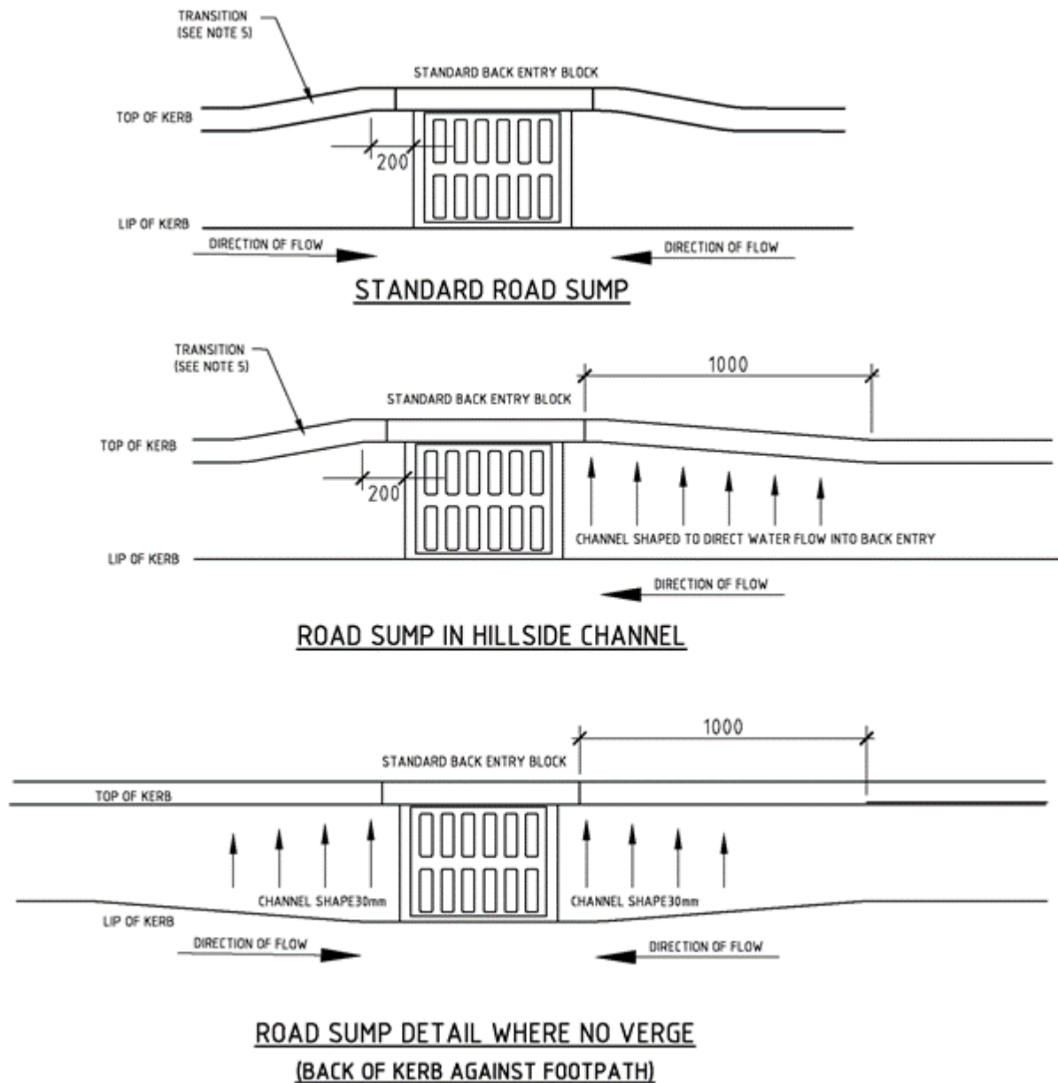
Drawing B5-12: Different Grate Layouts
