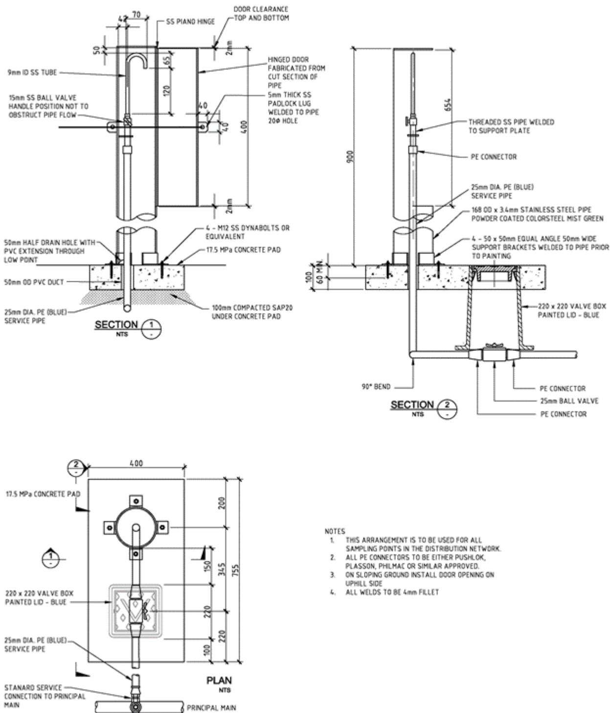
Drawing B2-9: Water Sampling Point
