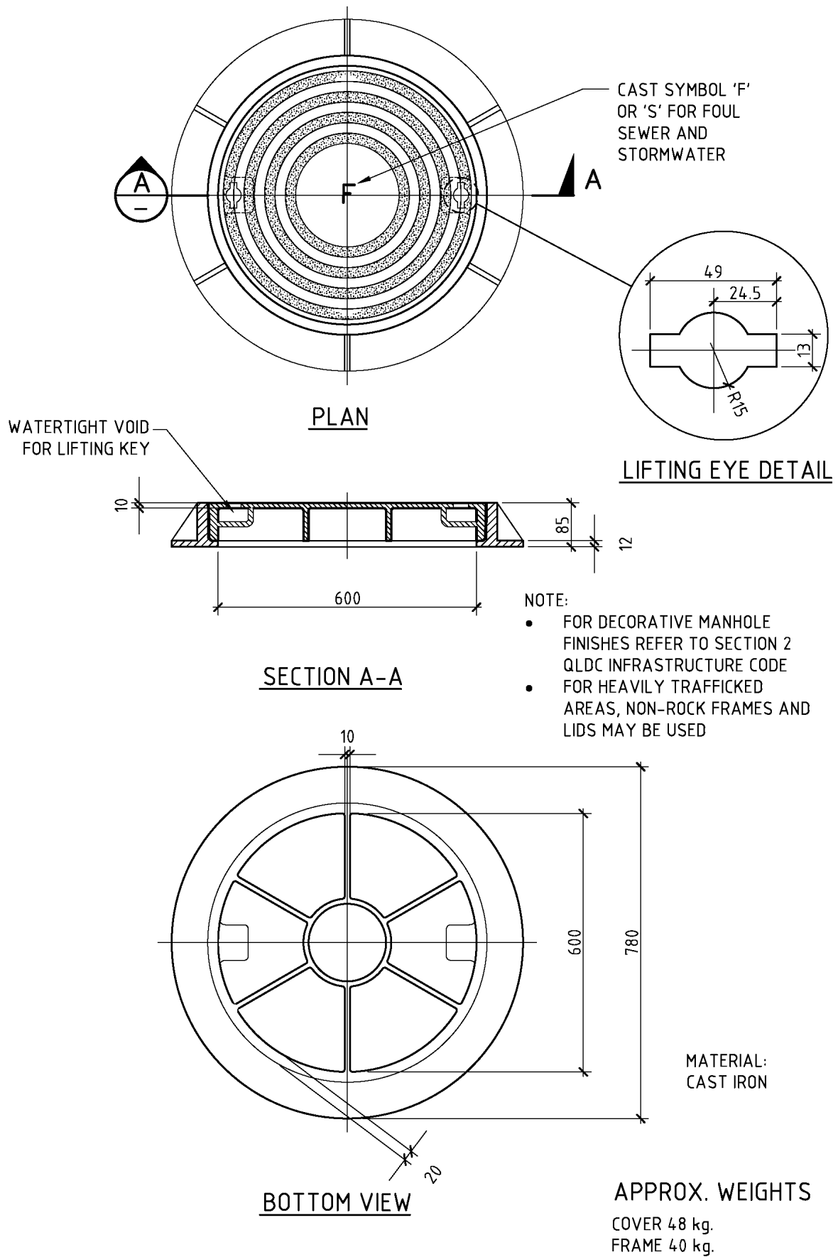
Drawing B1-13 Manhole: Typical Heavy Duty Frame & Lid
