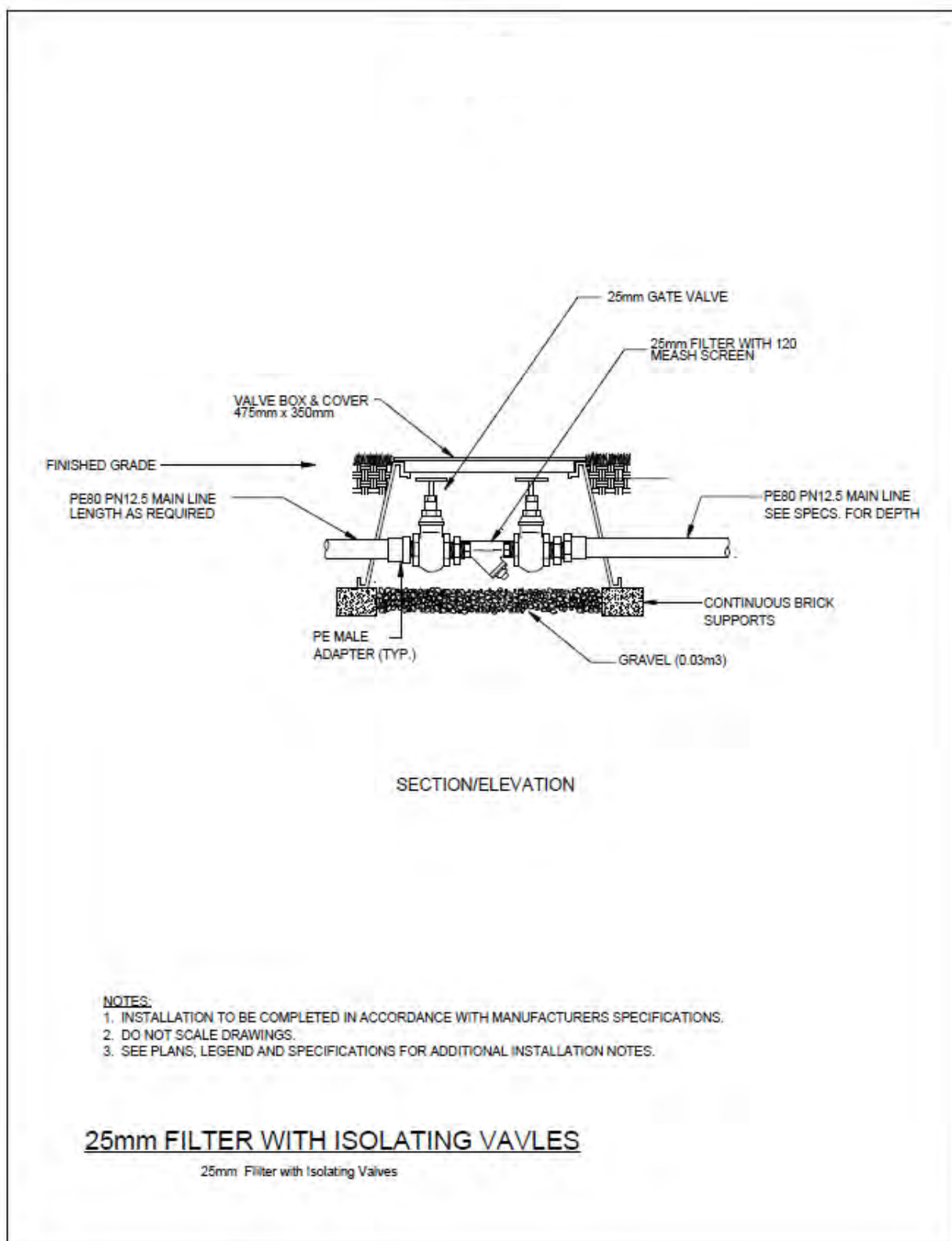
Drawing F0-4: Filter – 25mm
