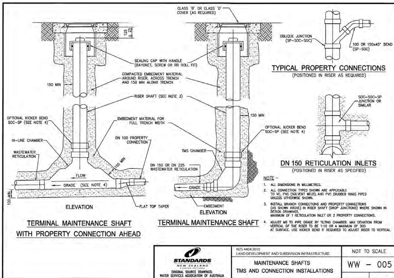
Drawing B7-12: WW - 005 Maintenance shafts - TMS and connection installations
