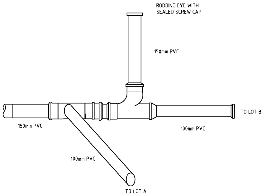
Drawing B1-12 Lateral Connections for two Properties
