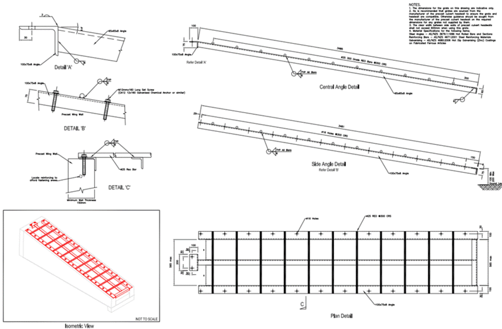
Drawing B5-17: Mountable Grates for Precast Headwalls 255mm to 450mm Culverts
