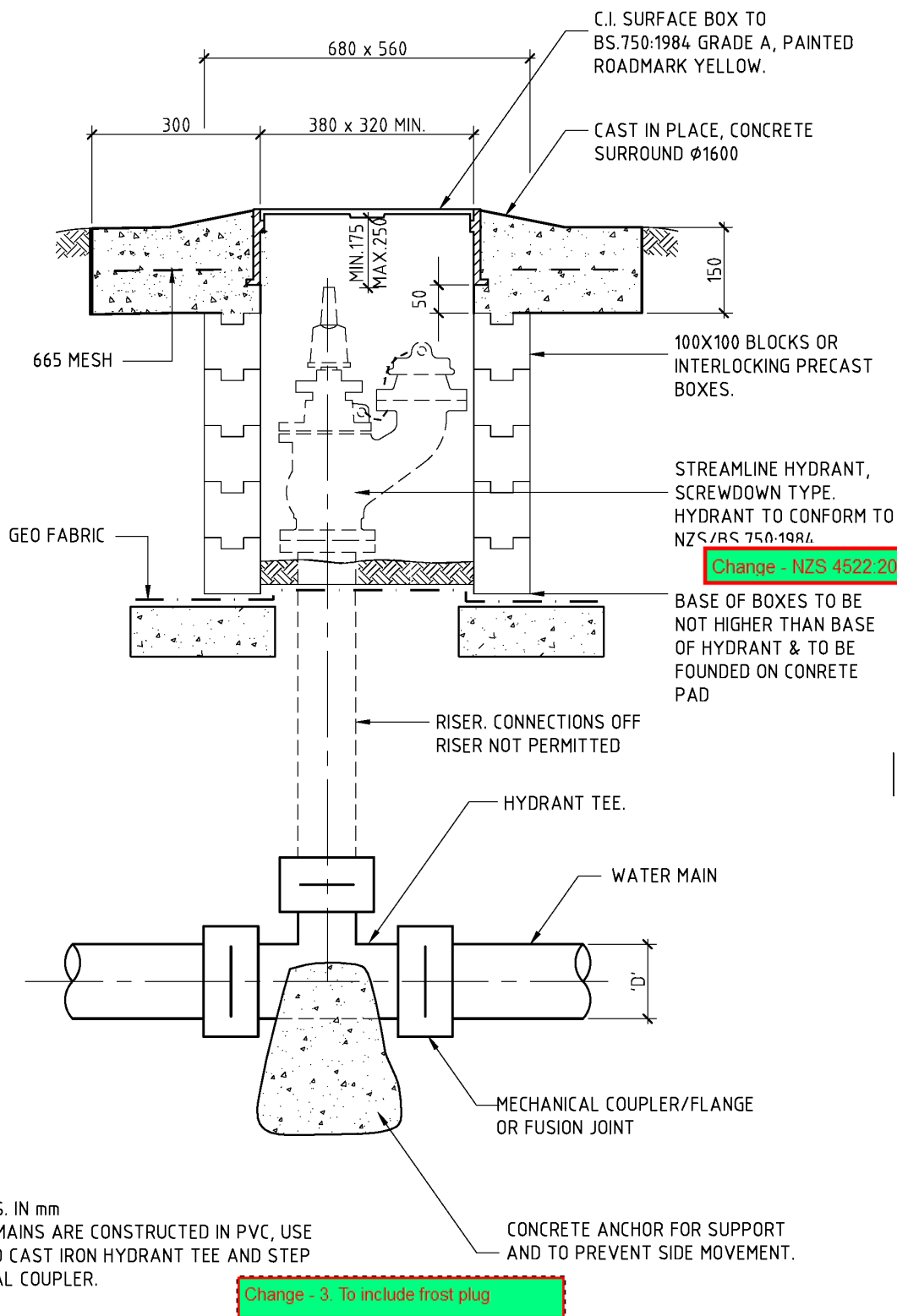
Drawing B2-1 Fire Hydrant
