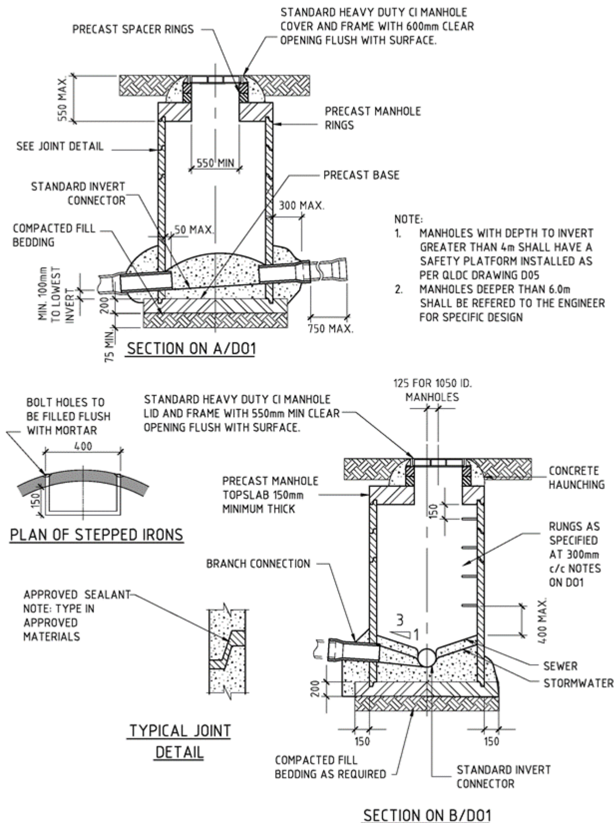
Drawing B1-10 Manhole Detail – Typical Cross Section
