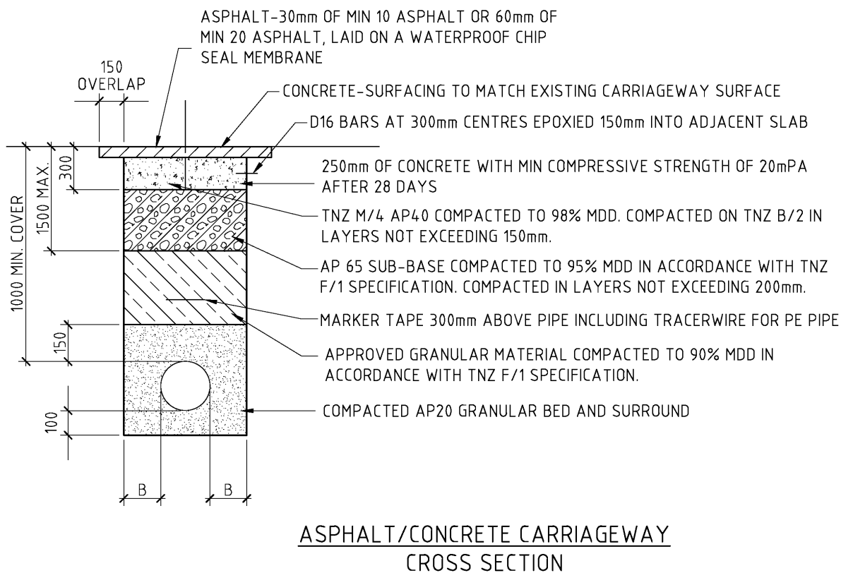
Drawing B1-3 Typical Pipe Bedding & Backfill for Carriageways
