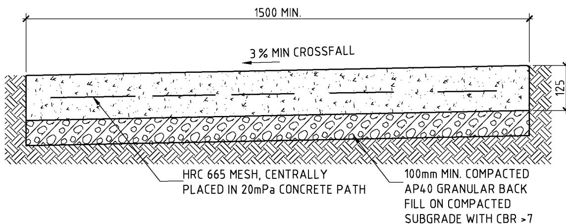
Drawing B5-24: Heavy Duty Footpath
