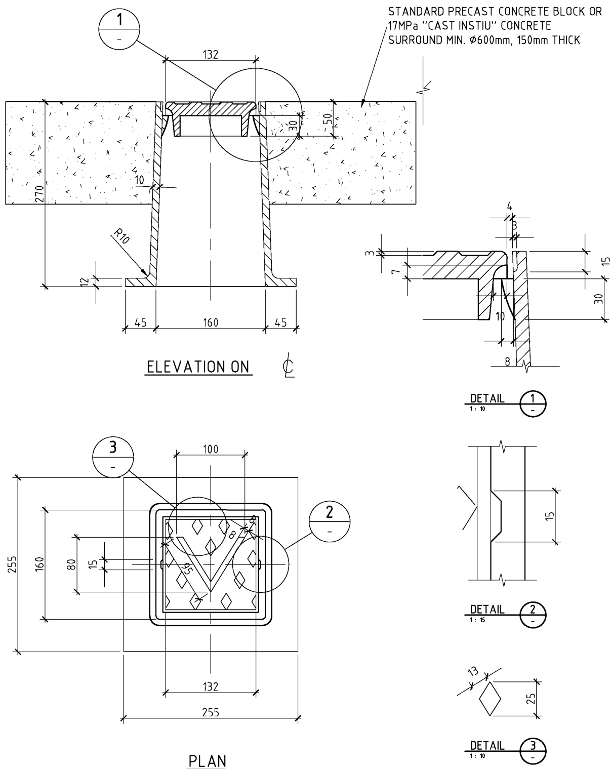
Drawing B2-3 Typical Cast Iron Valve Box
