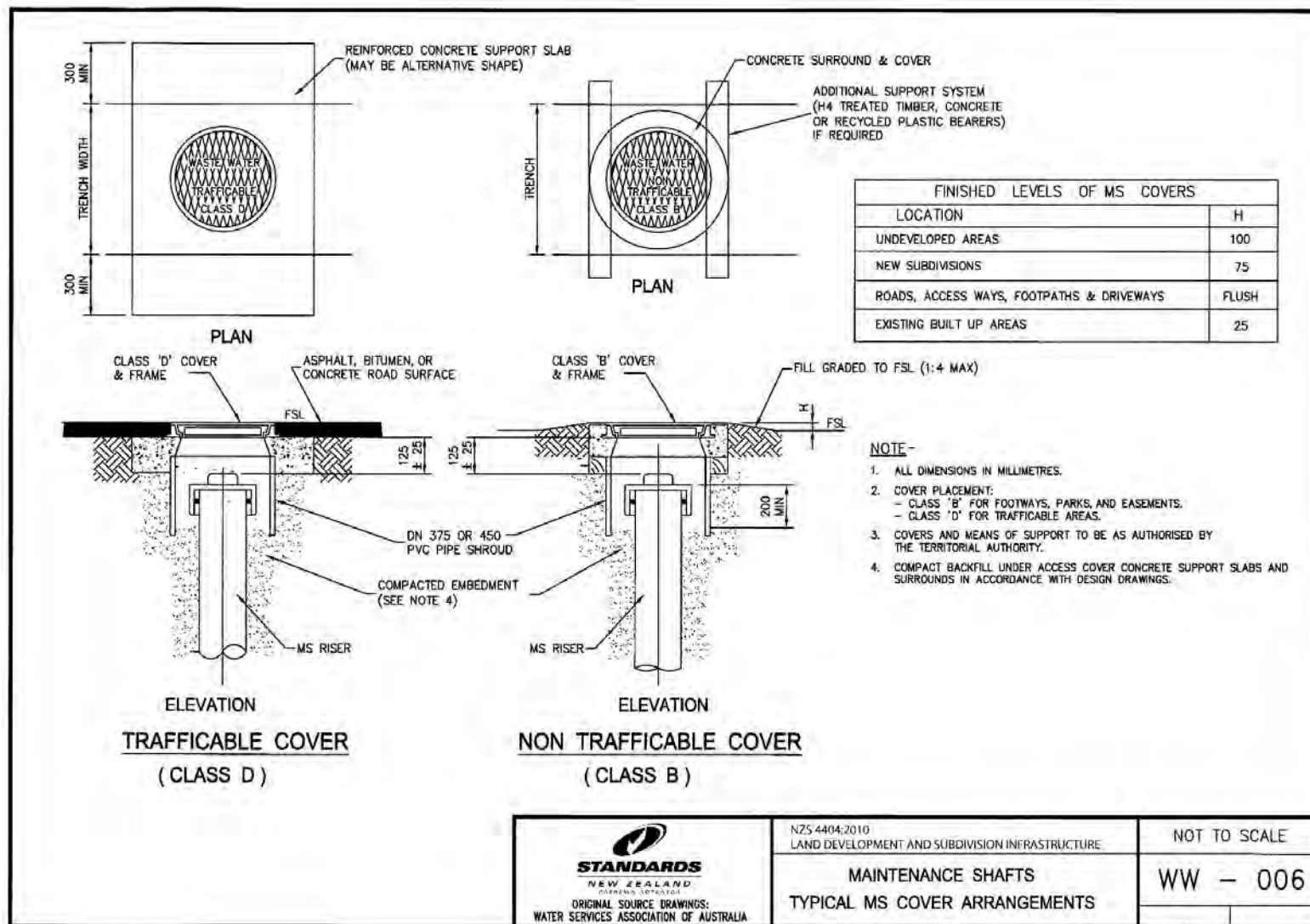
Drawing B7-13: WW – 006 Maintenance shafts – Typical MS cover arrangements
