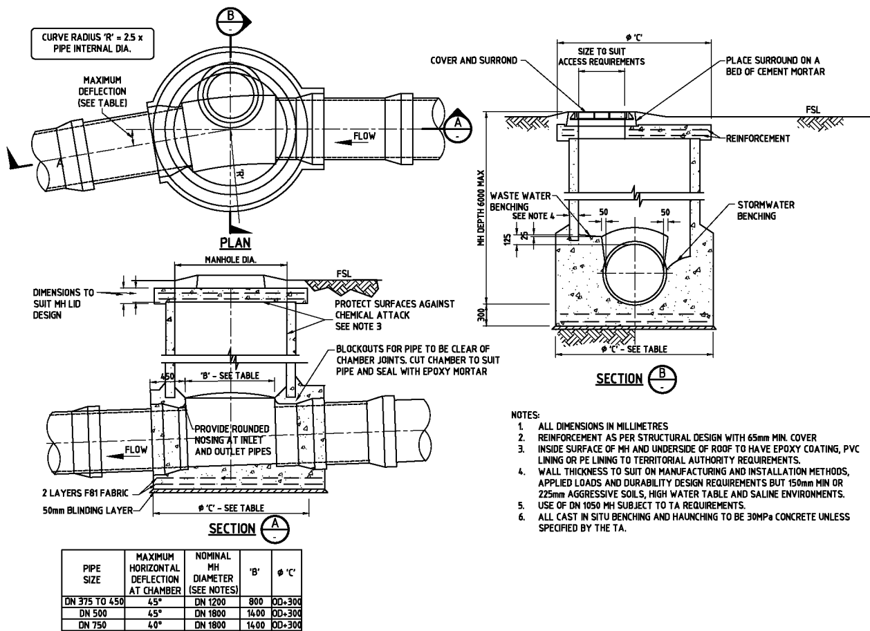
Drawing B1-9 Stormwater or Wastewater DN375 to DN750
