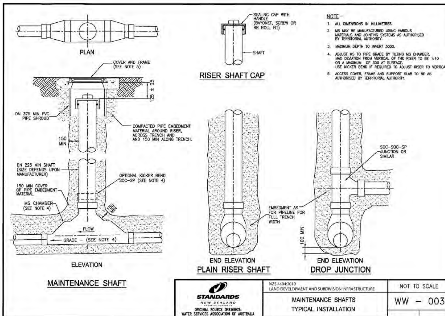
Drawing B7-10: WW - 003 Maintenance shafts - Typical installation
