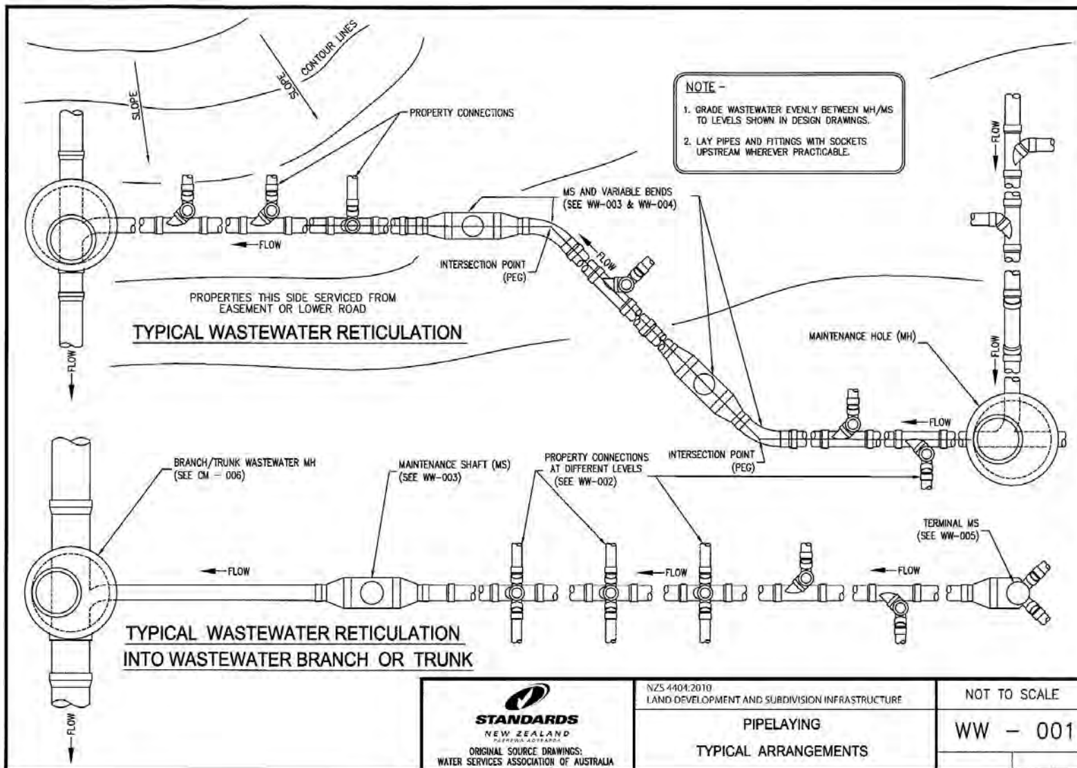
Drawing B7-8: WW – 001 Pipelaying – Typical arrangements
