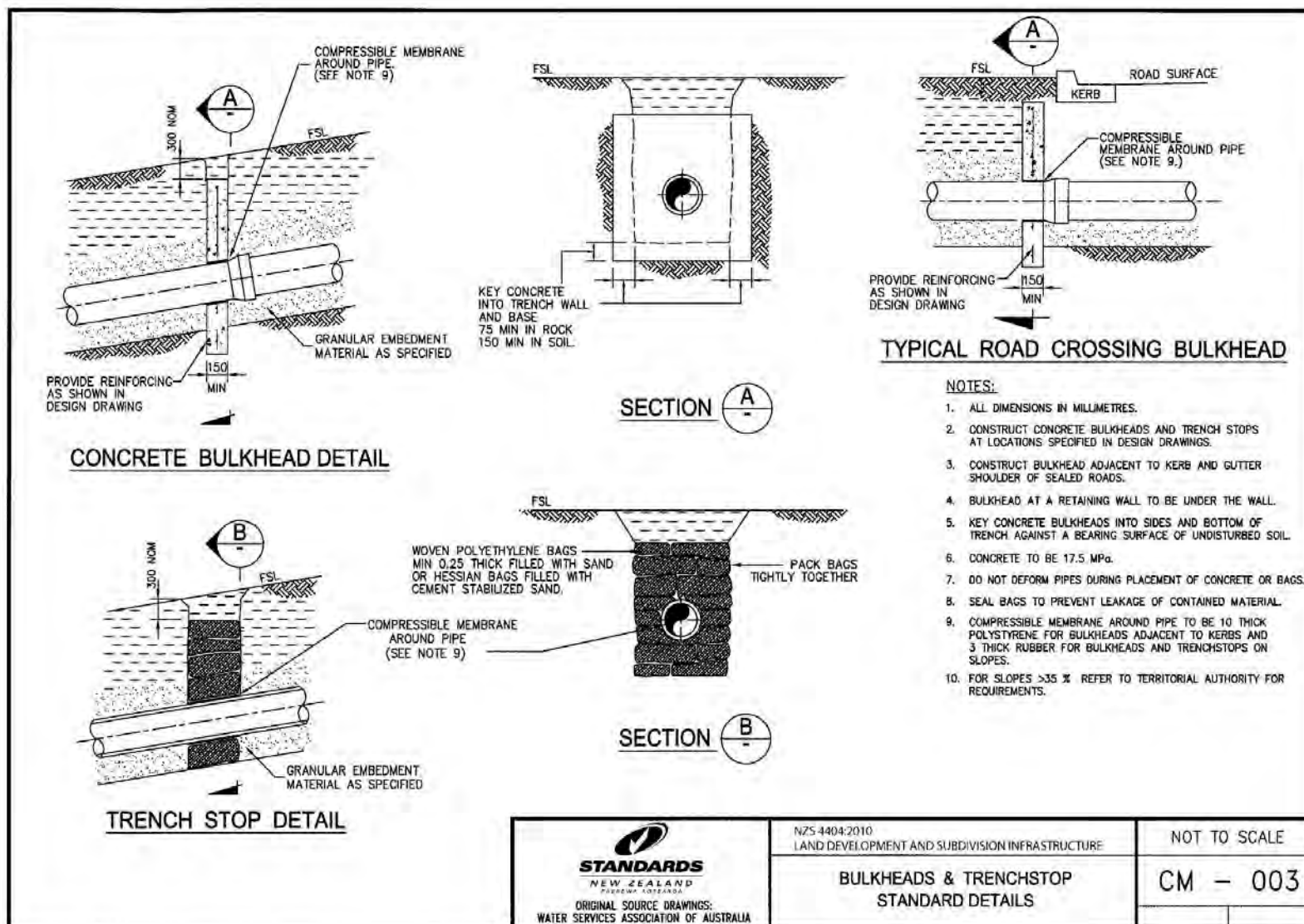
Drawing B7-2: CM003 Bulkheads & Trench stop Standard Details
