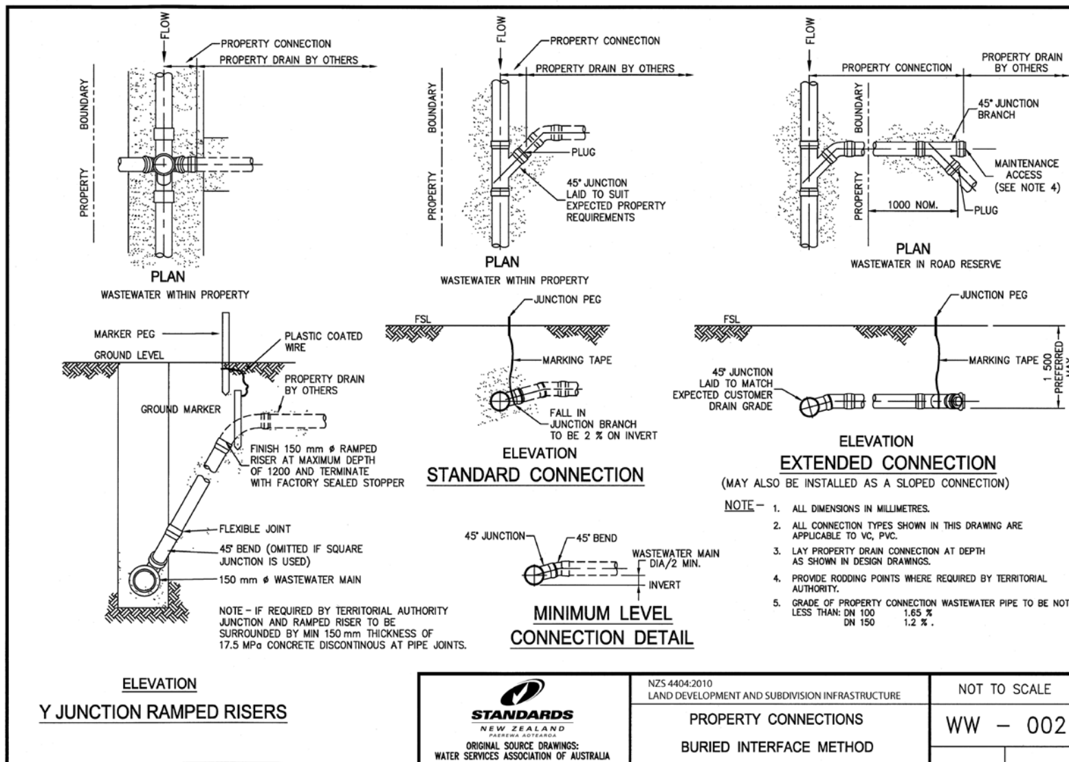
Drawing B7-9: WW - 002 Property connections - Buried interface method
