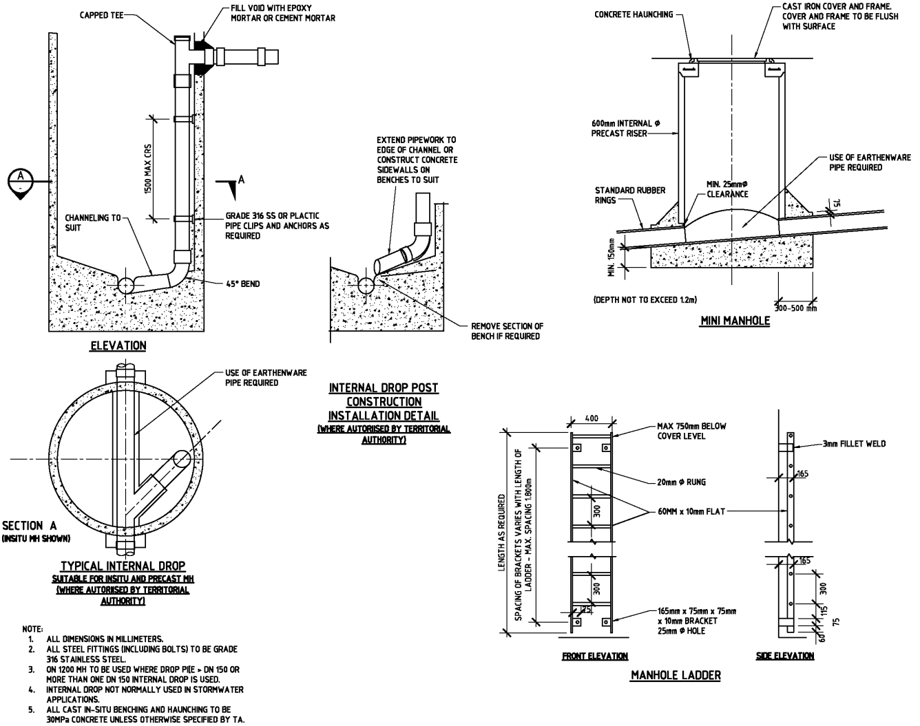
Drawing B1-8 Mini & Drop Manhole Detail
