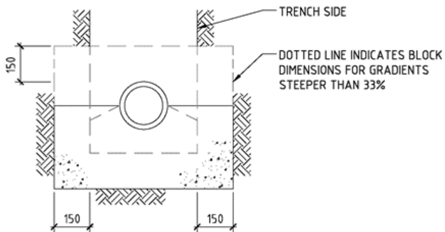
CROSS SECTION
