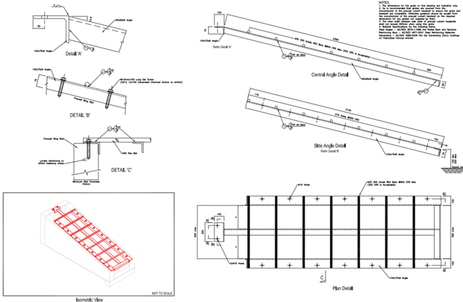
Drawing B5-16: Traversable Grates for Precast Headwalls 255mm to 450mm culverts
