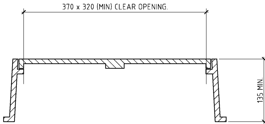
SECTION THROUGH FRAME AND COVER
