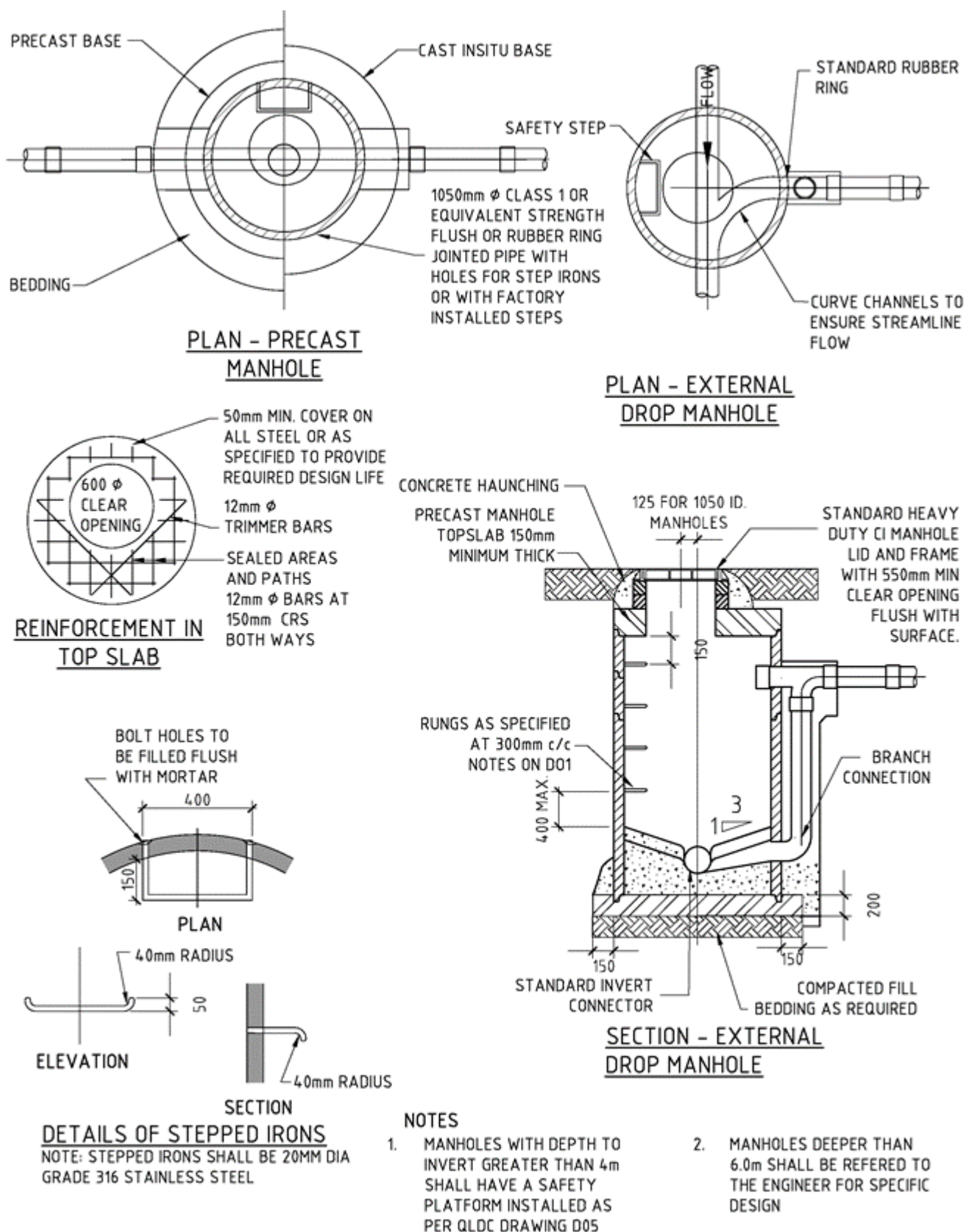
Drawing B1-7 Manhole Detail C
