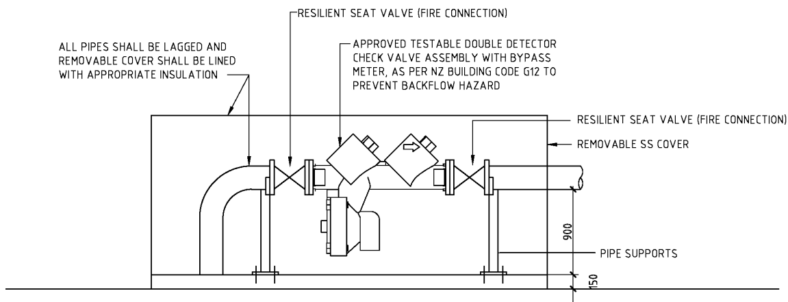
SIDE ELEVATION
