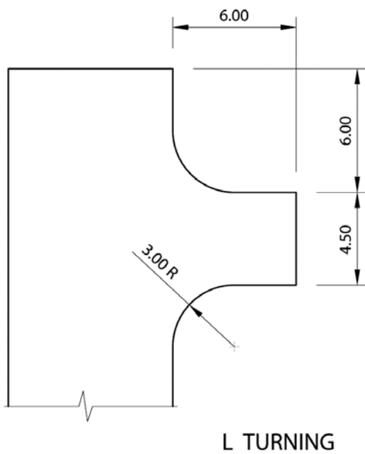
Drawing B5-2: Turning Areas for No-Exit Roads
