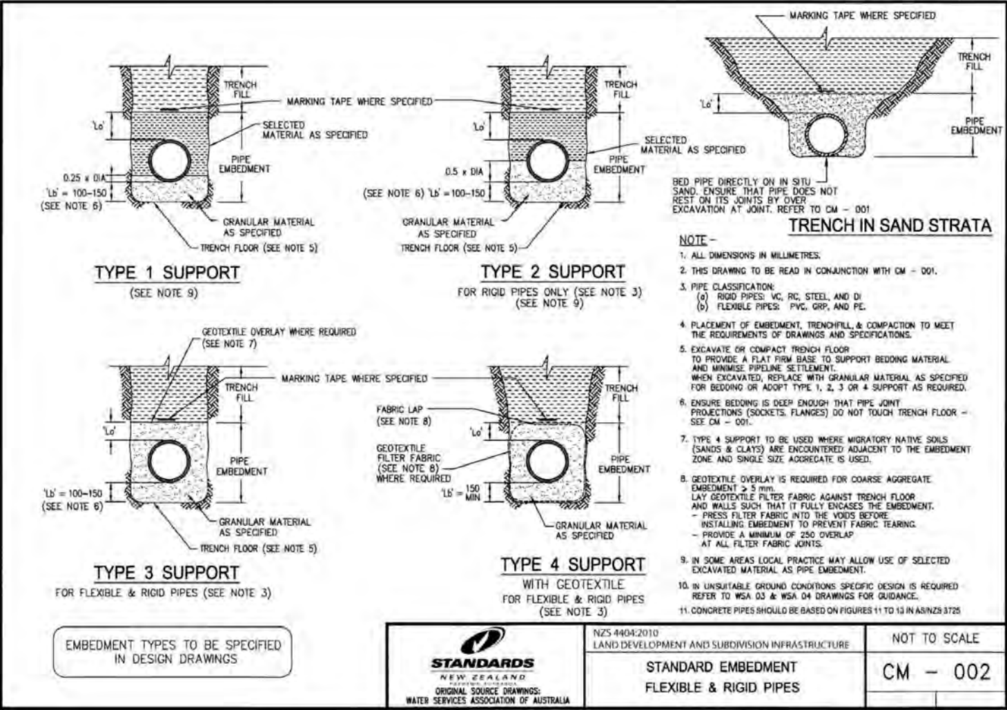
Drawing B7-1:CM - 001 Embedment & Trenchfill Arrangement
