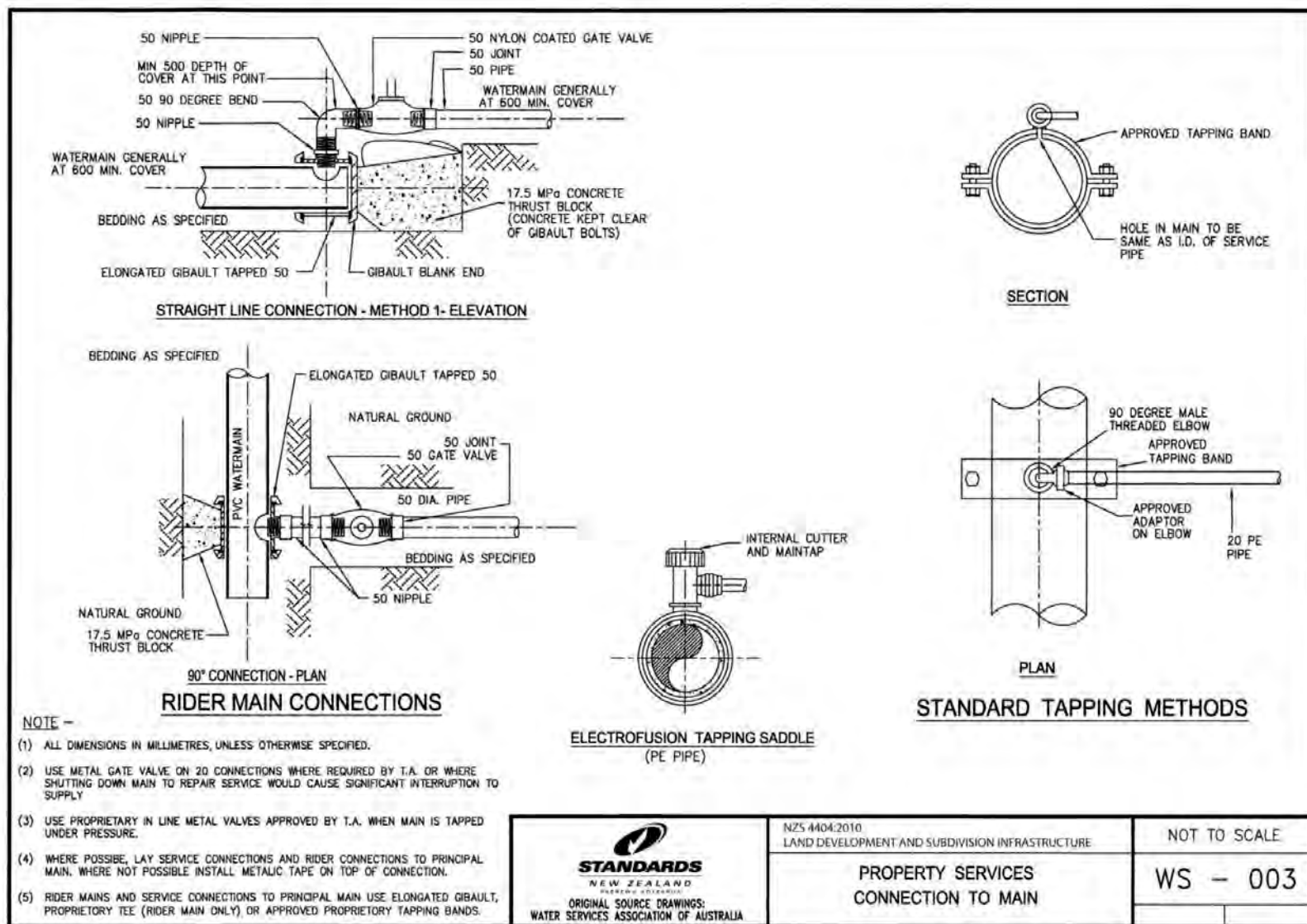
Drawing B7-5: WS – 003 Property Services – Connection to Main
