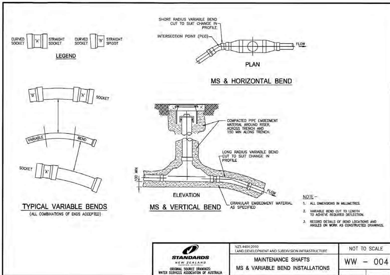
Drawing B7-11: WW – 004 Maintenance shafts – MS and variable bend installations
