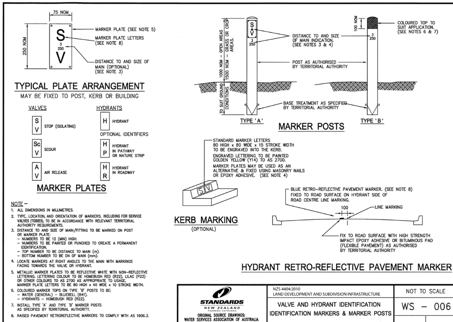
Drawing B7-7: WS – 006 Valve And Hydrant Identification Marker Posts
