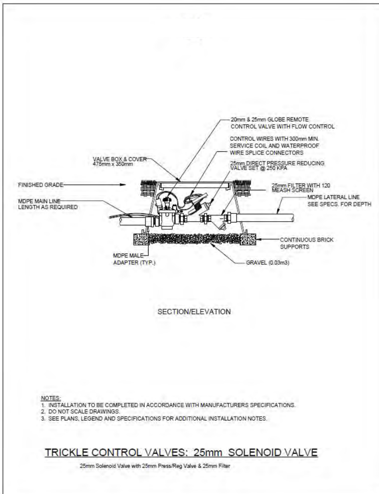
Drawing F0-5: Trickle Control 25mm
