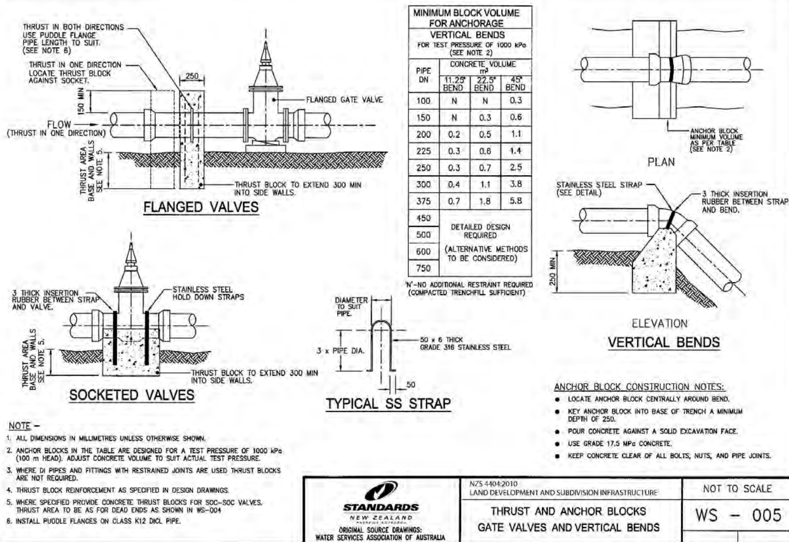
Drawing B7-6: WS - 005 Thrust and anchor blocks - Gate valves and vertical bends
