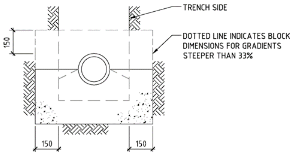
CROSS SECTION
