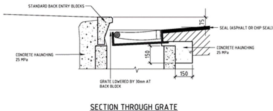
Drawing B5-13: Standard Section Through Grate
